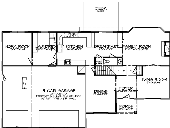
FIRST FLOOR PLAN A-4
