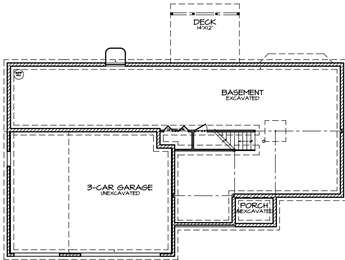
FOUNDATION PLAN A-3
